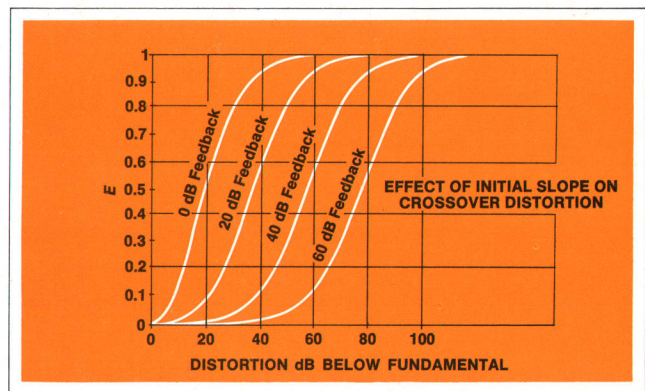
Fig. 14. Effect of initial slope on crossover distortion.
